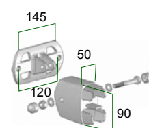
Soporte terminal regulable
